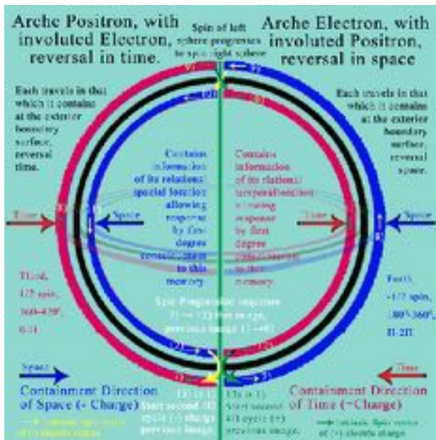
Image V 2\pi \Rightarrow 3/4\pi left side, 3/4\pi \Rightarrow 4\pi right. Sequence 7) - 12) both charges both dimensions.
